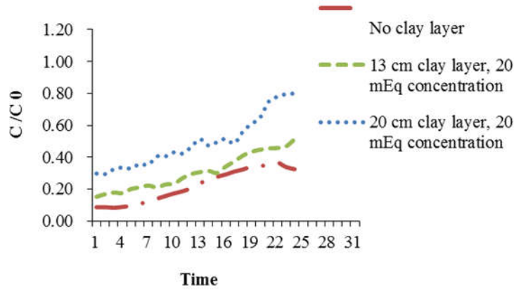
Fig. 9. Intrusion curve for bellows and clay layers for 20 mEq/l of salt
